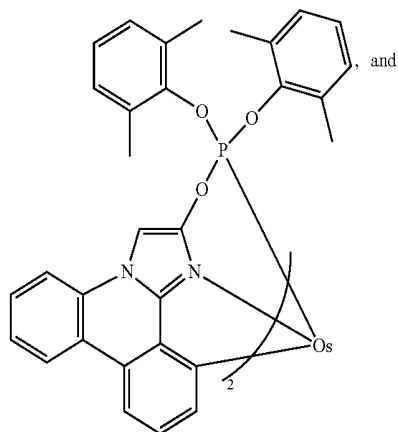
Compound 18
