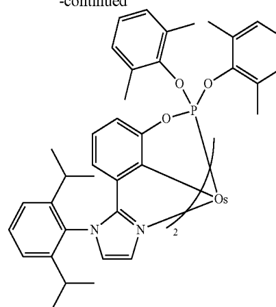
CPD.1
