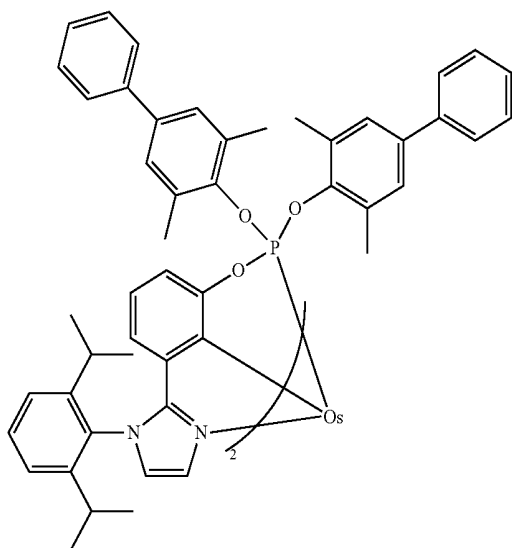
Compound 11
