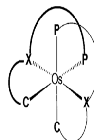
FORMULA II
