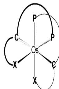
FORMULA I
