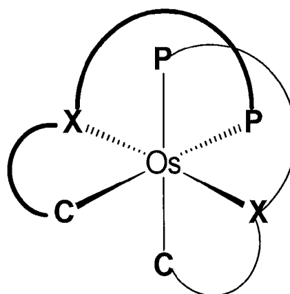
FORMULA II
