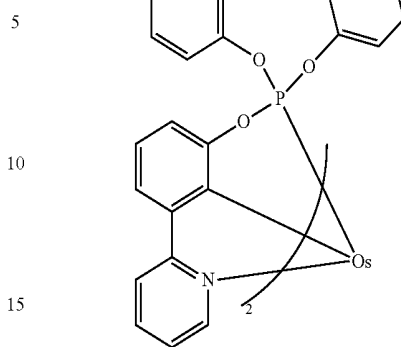
Compound 1
