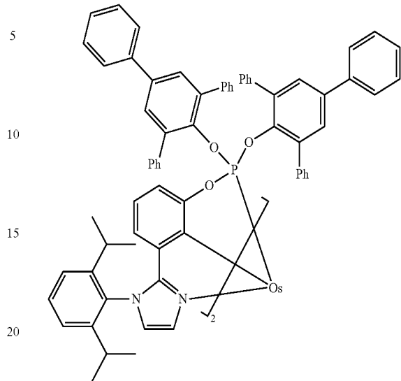
Compound 12
