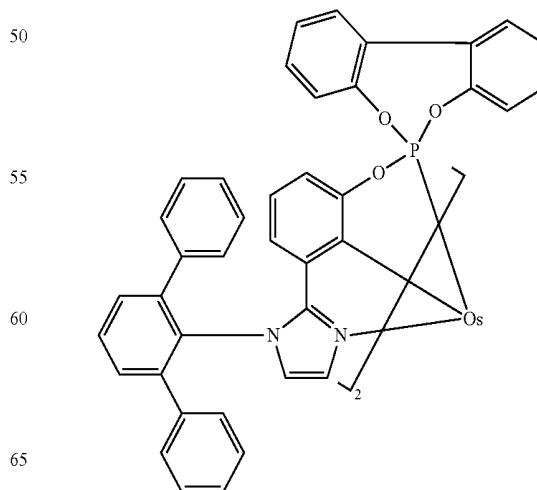
Compound 14
